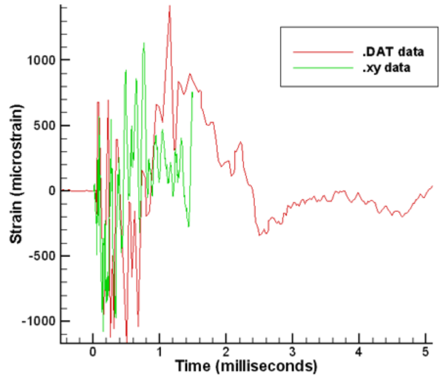
Output Strain214.dat
