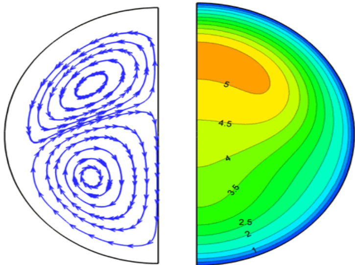
Natural Convection of water in a circular enclosure (Stream lines, and Temp. Contours)
